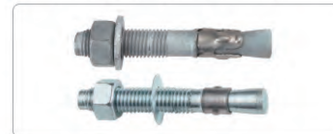
H.D.G Wedge Anchor With SS A2/A4 Clip
